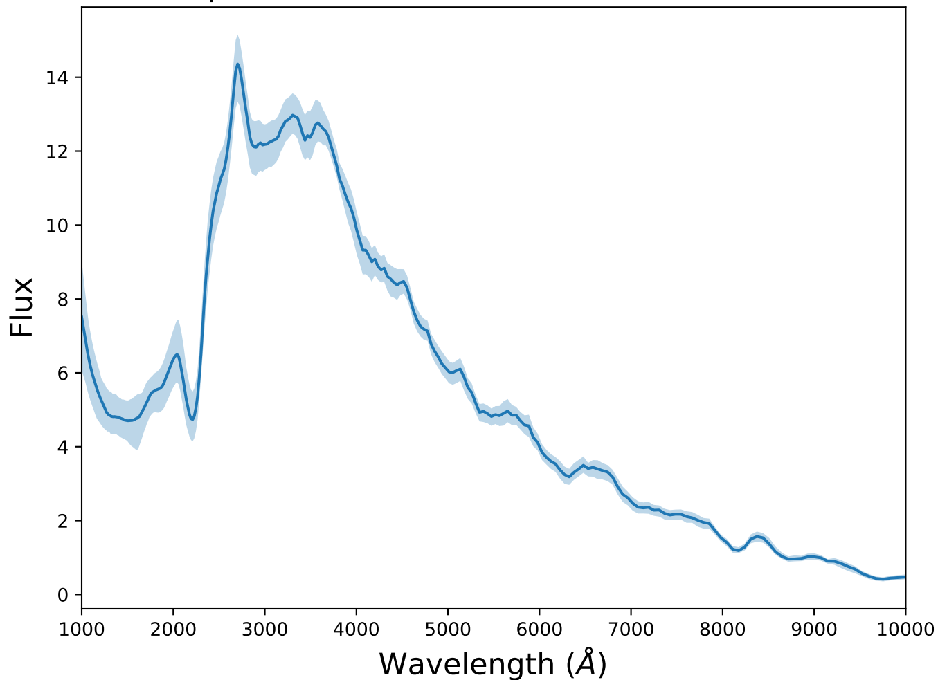
Spectrum 2 for transient CCSN at z=1.13
